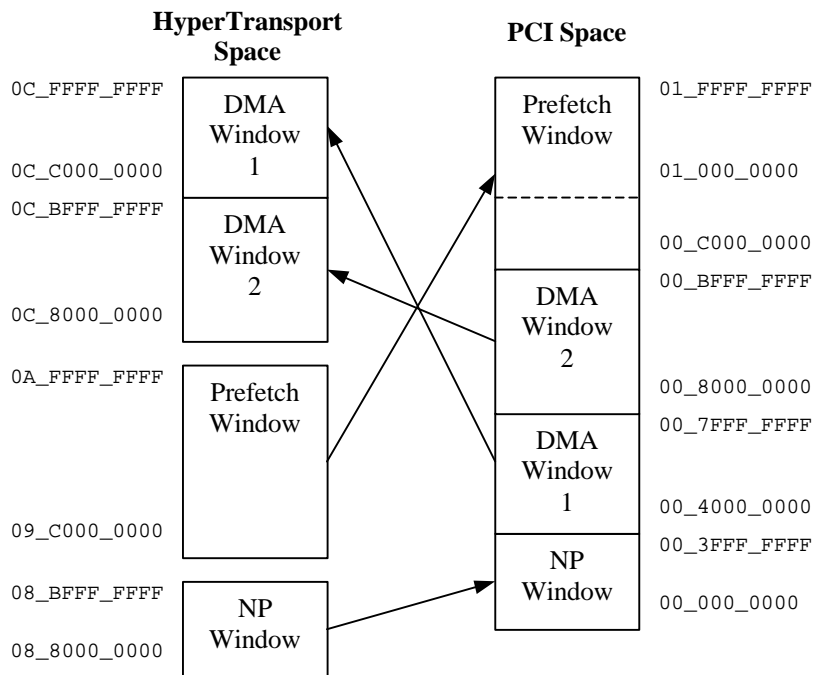
Figure 8. DMA Window Remapping
