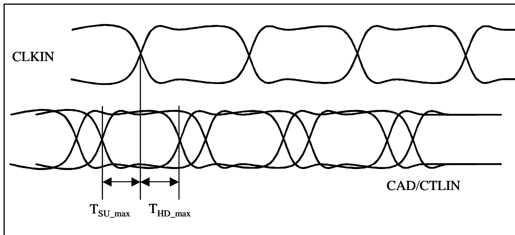
Figure 24. T_{SU} and T_{HD}
