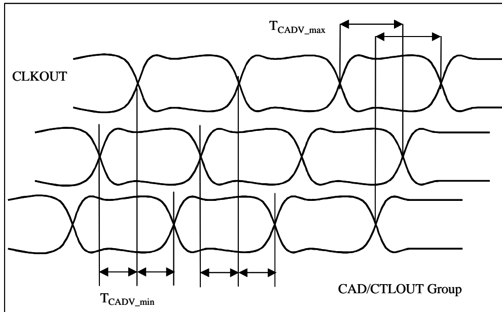
Figure 22. T_{CADV}
