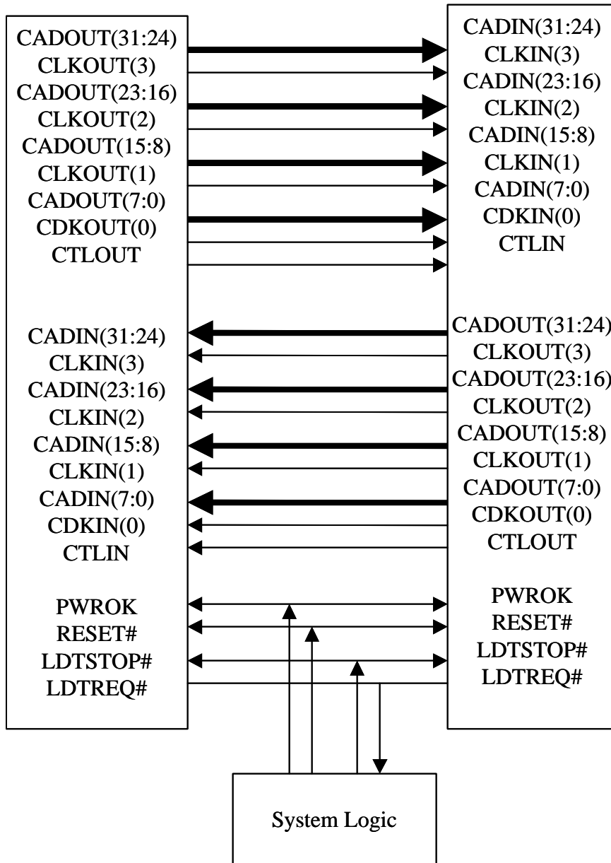
Figure 9. HyperTransport™ Link Interconnect
