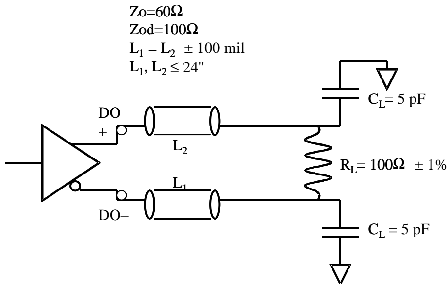
Figure 15. AC Reference System Load for Links up to 800 MT/s
