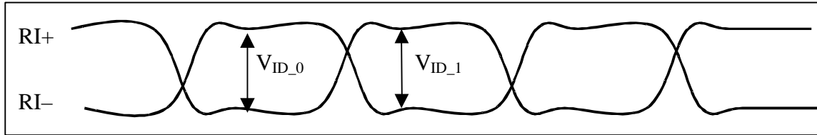
Figure 13. V_{ID} DC
