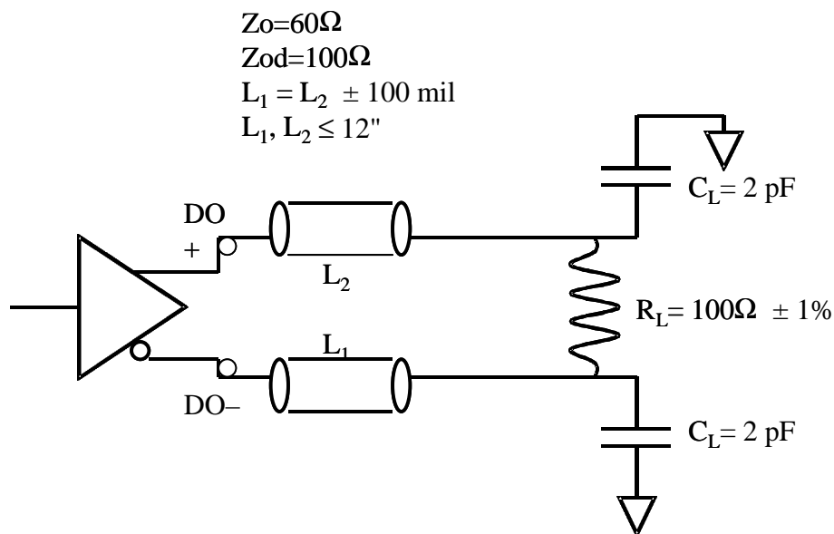
Figure 16. AC Reference System Load for Links Above 800 MT/s
