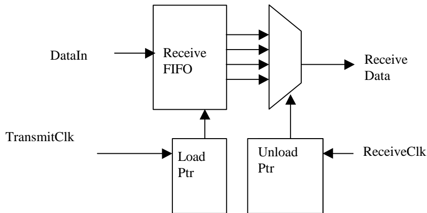
Figure 5. Receive FIFO
