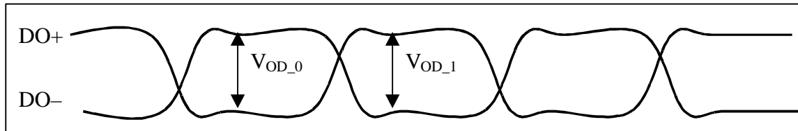
Figure 17. V_{OD} AC
