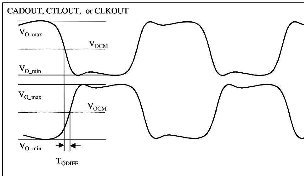
Figure 21. T_{ODIFF}
