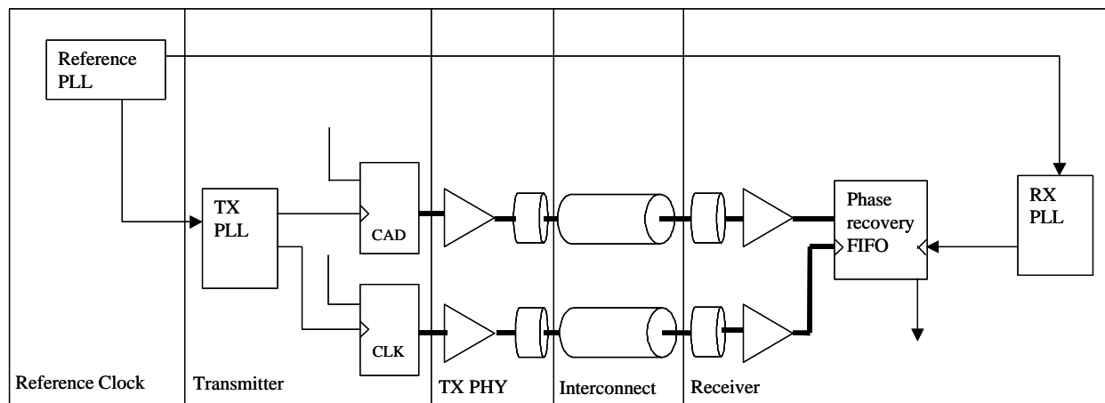
Figure 27. Representative Transmitter and Receiver
