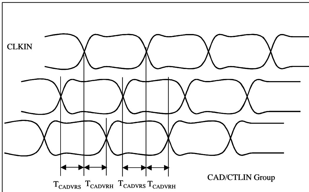
Figure 25. T_{CADVRS}/T_{CADVRH}
