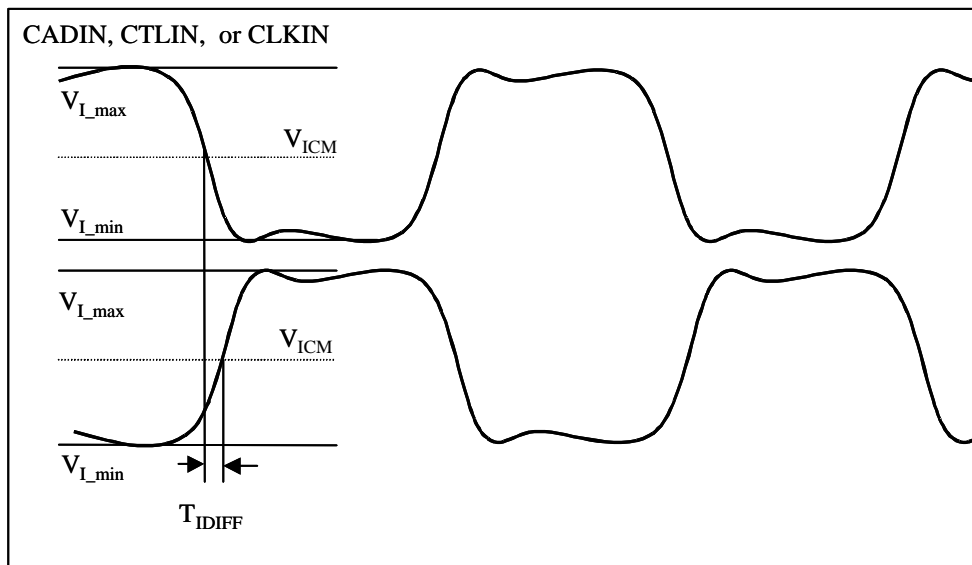
Figure 23. T_{IDIFF}
