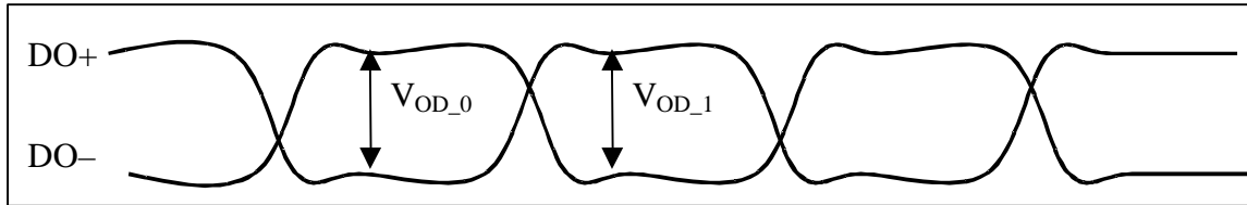
Figure 11. V_{OD}DC
