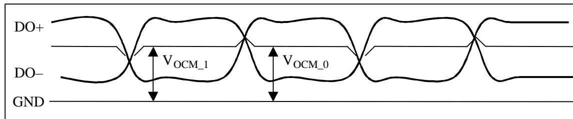
Figure 18. V_{OCM} AC
