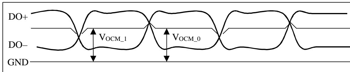
Figure 12. V_{OCM}DC
