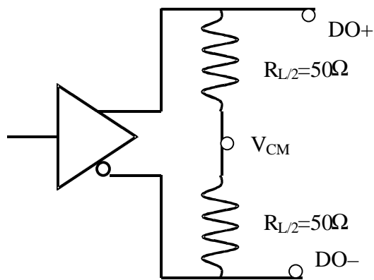
Figure 10. DC Output Reference System Load
