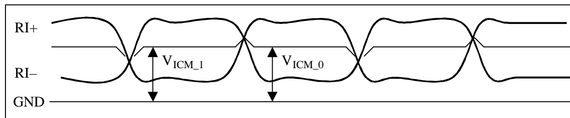
Figure 20. V_{ICM} AC
